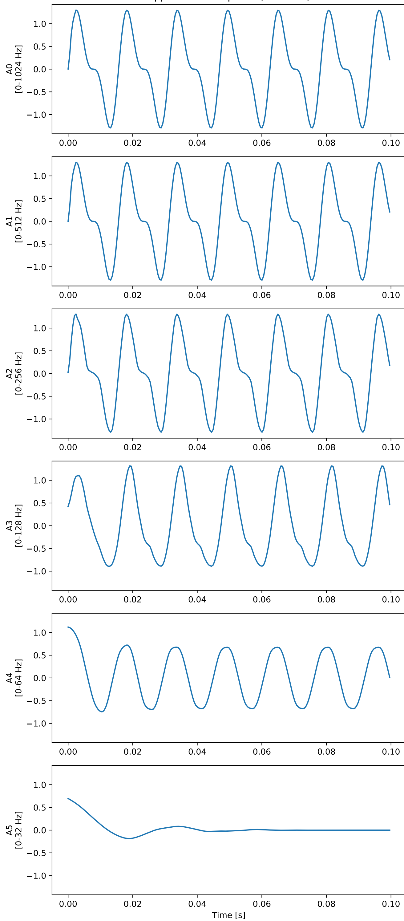
Approximation spaces (modified)
