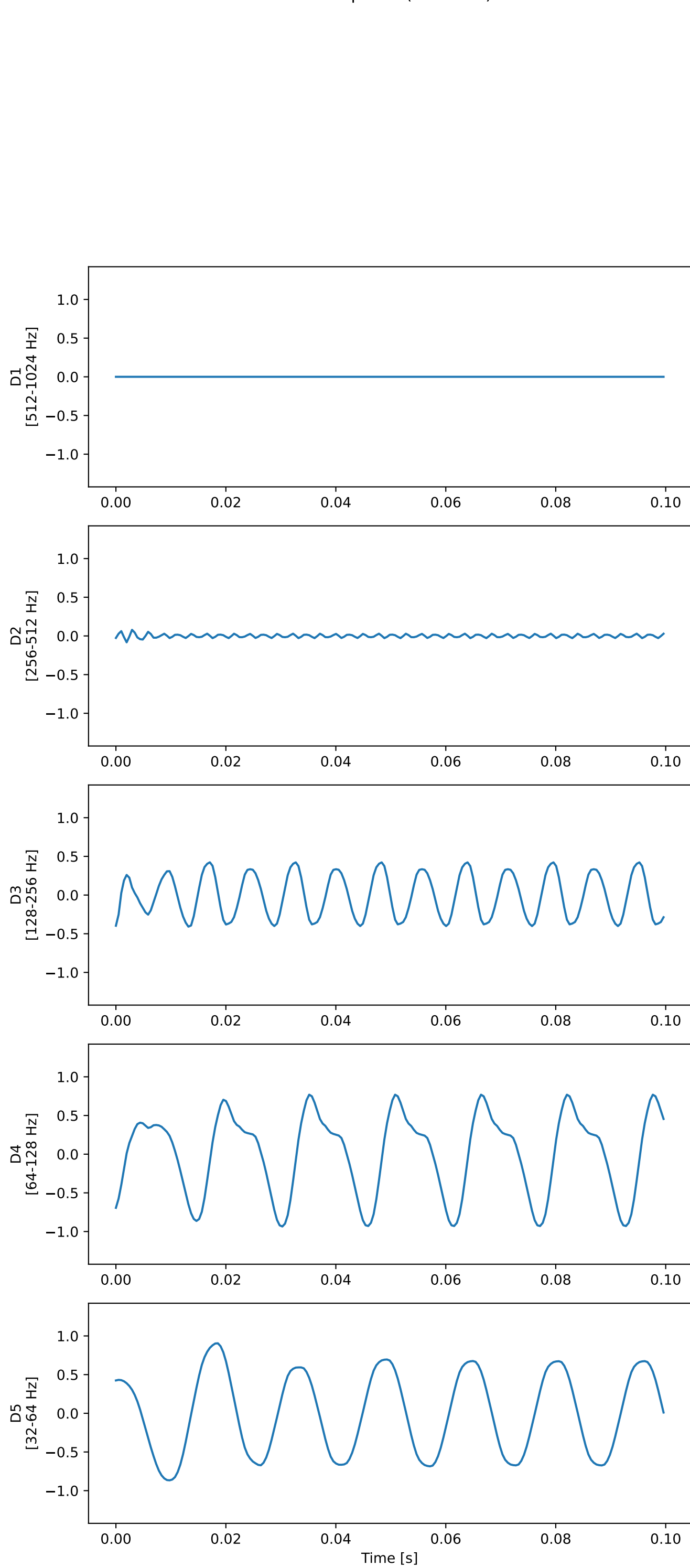
Detail spaces (modified)
